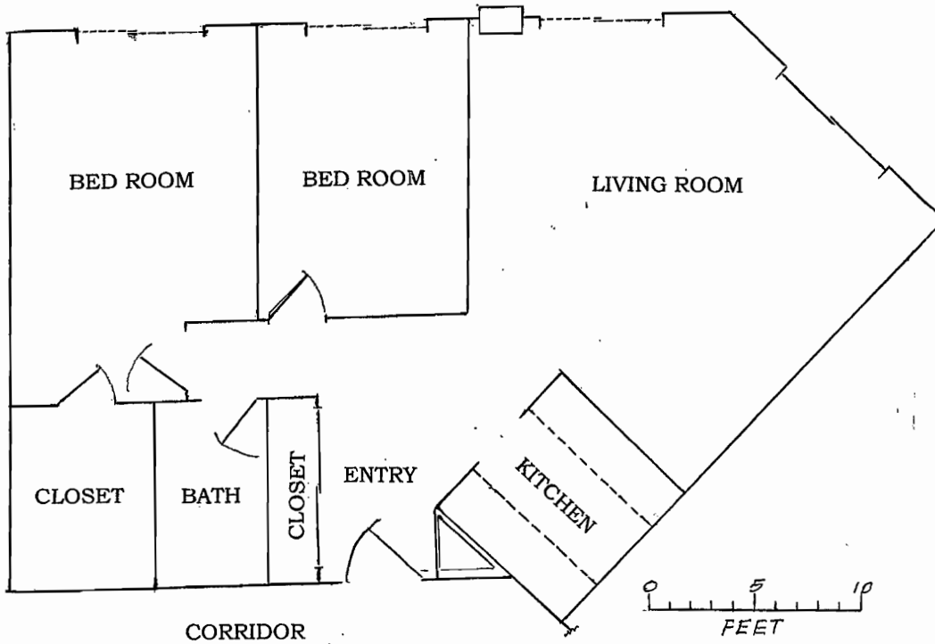
TYPICAL E' - APARTMENT THERE MAY BE SLIGHT VARIATIONS IN OTHERS
